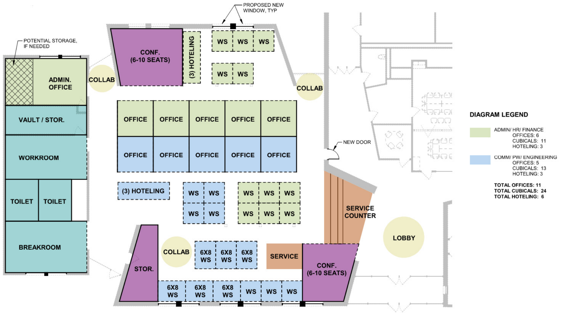
PROPOSED MAIN LEVEL PLAN – BUBBLE DIAGRAM
