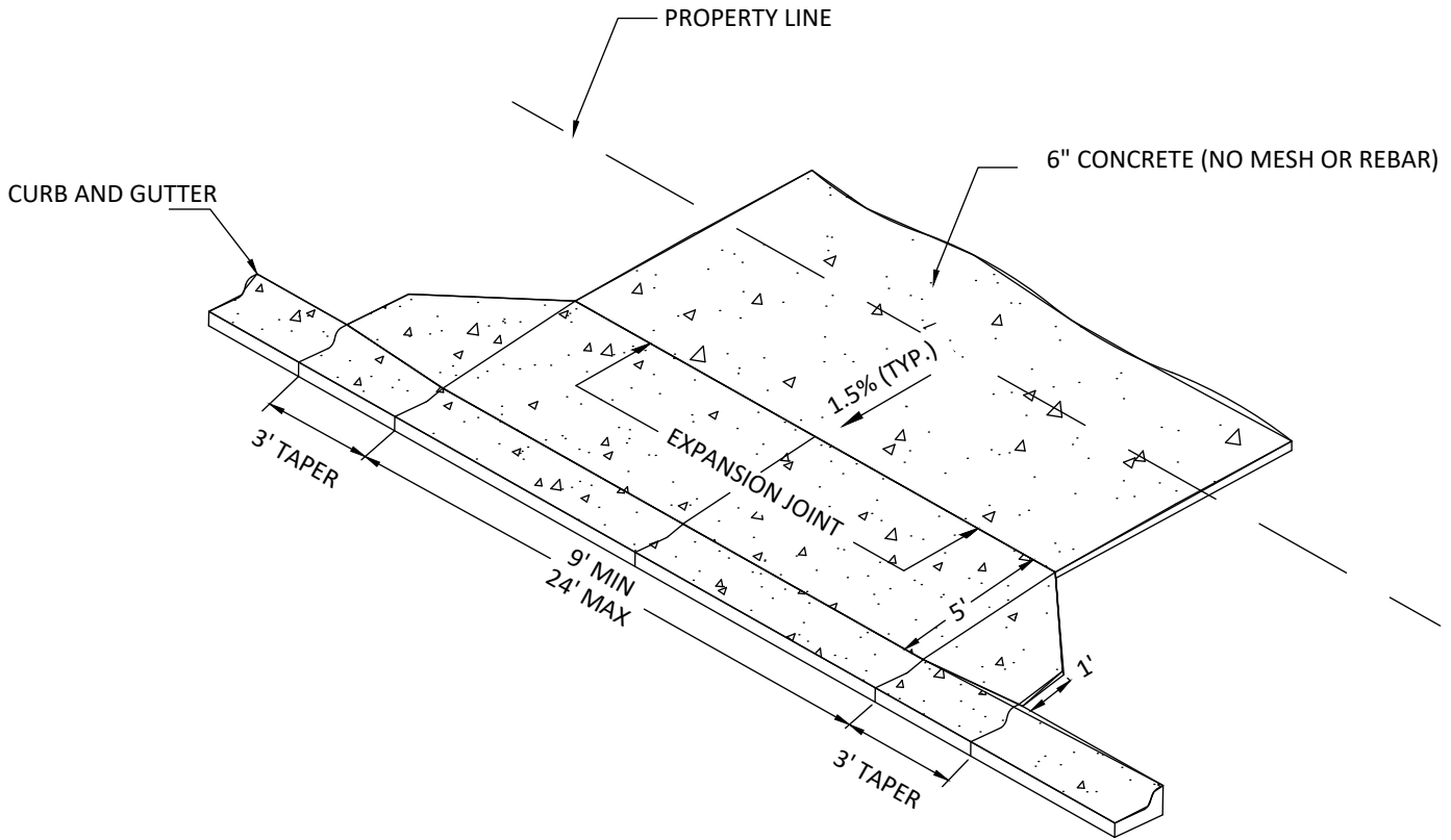
ISOMETRIC
