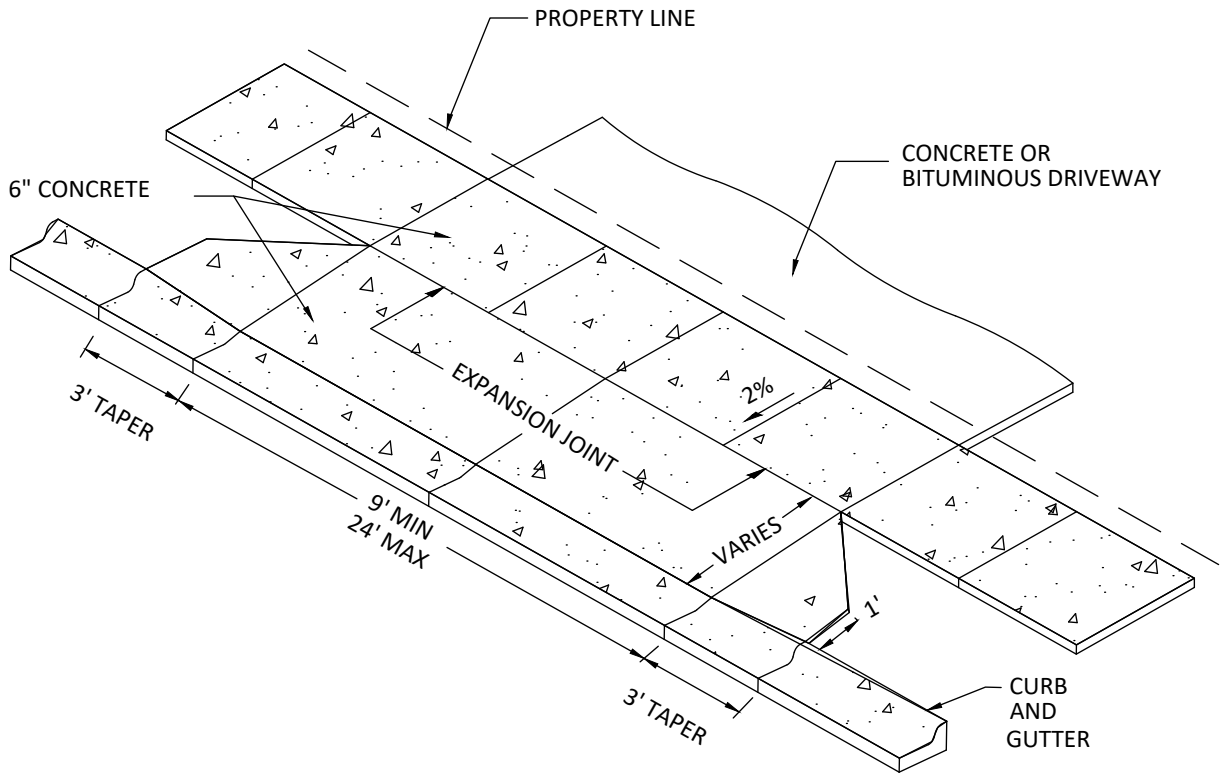
ISOMETRIC
